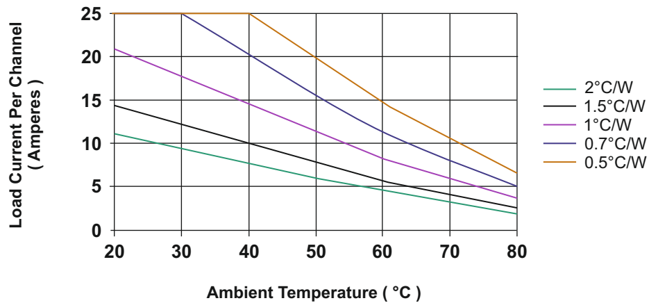
DERATE CURVES 29 Series IP20 25A
